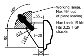
B (1:5)
