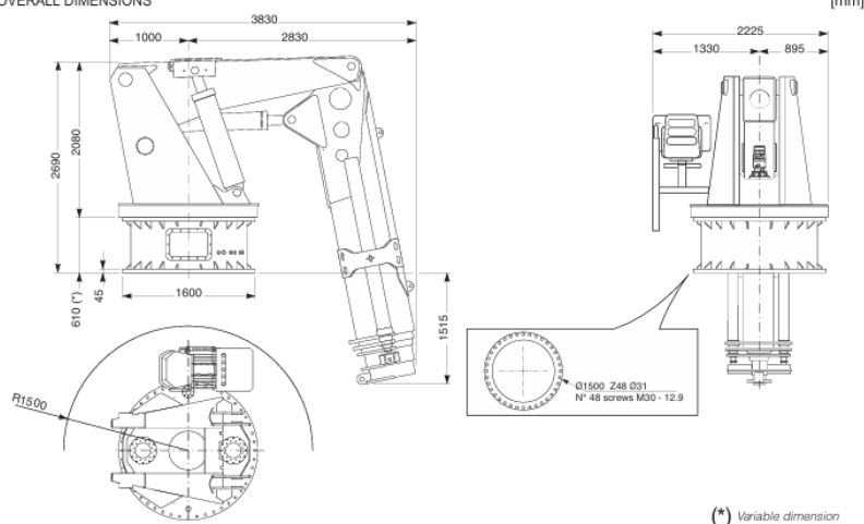
OVERALL DIMENSIONS
